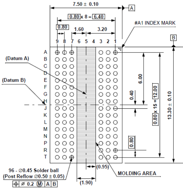
BOTTOM VIEW
