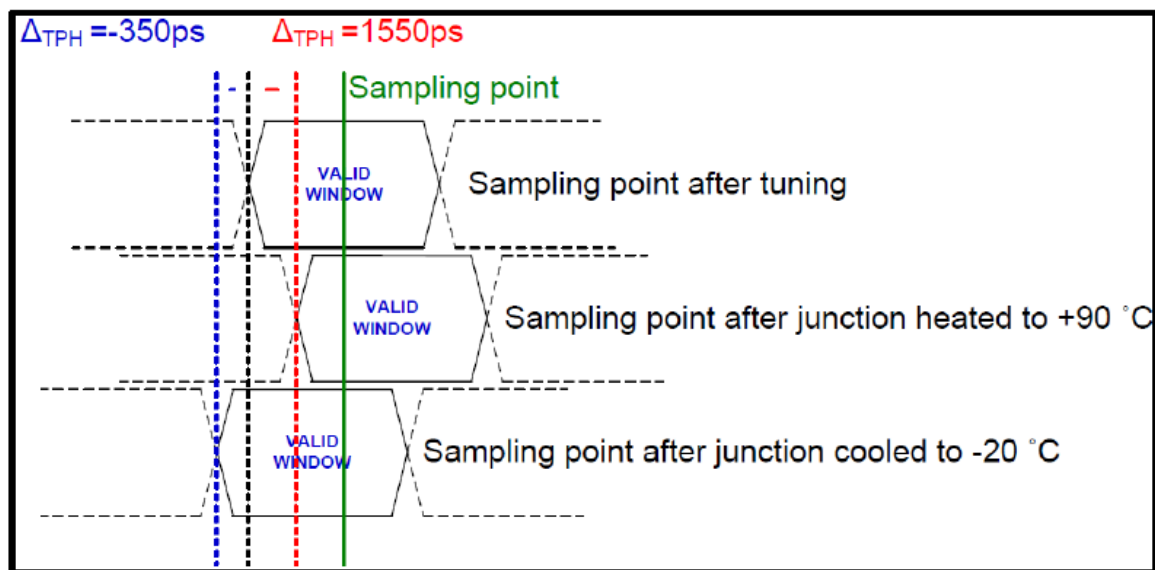
\Delta_{TPH} consideration
