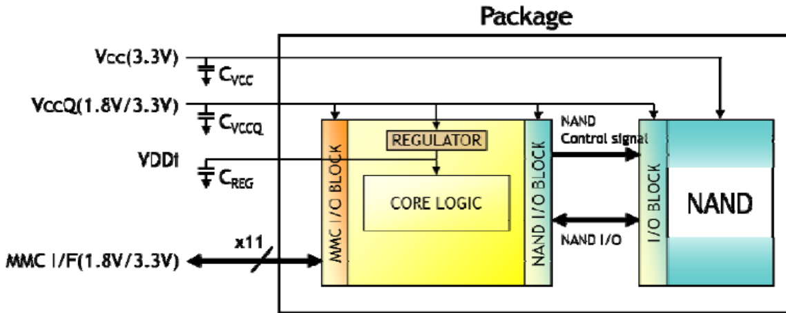
HAA18G35111I Block Diagram
