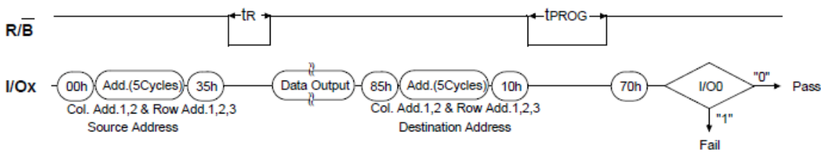
Copy-Back Program Sequence
