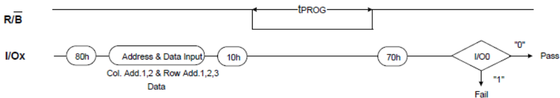
Page Program Sequence
