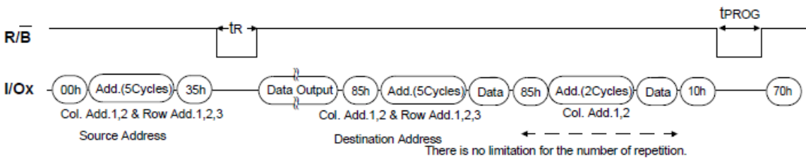
Copy-Back Program with Random Data Input Sequence
