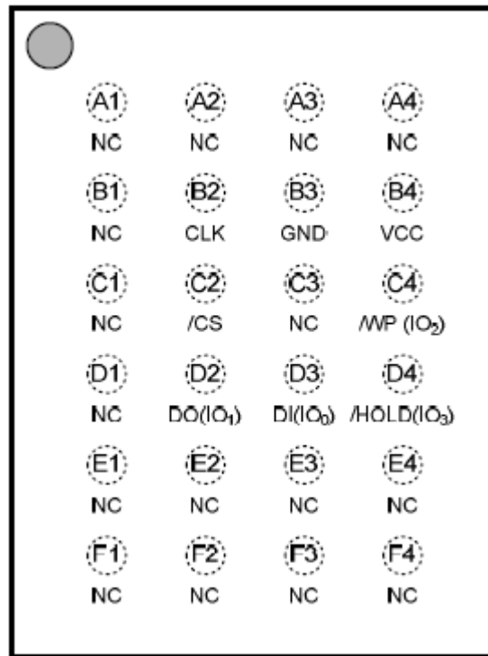
24-ball TFBGA 8x6mm(6x4 array)
