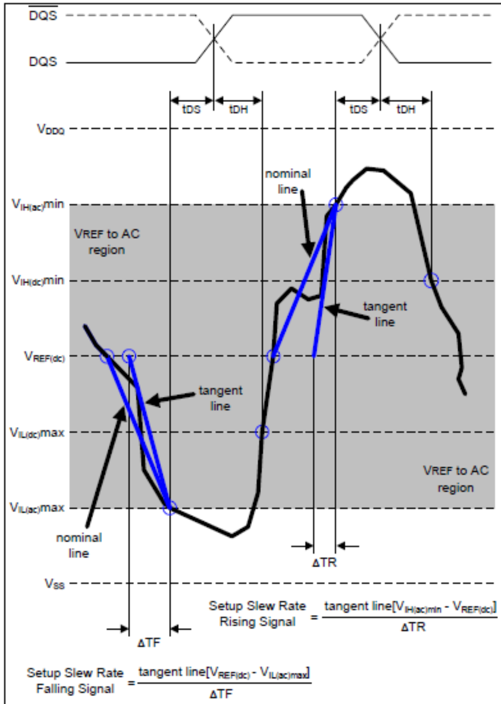
Figure 6 – Illustration of tangent line for tDS (differential DQS, \overline{DQS} )
