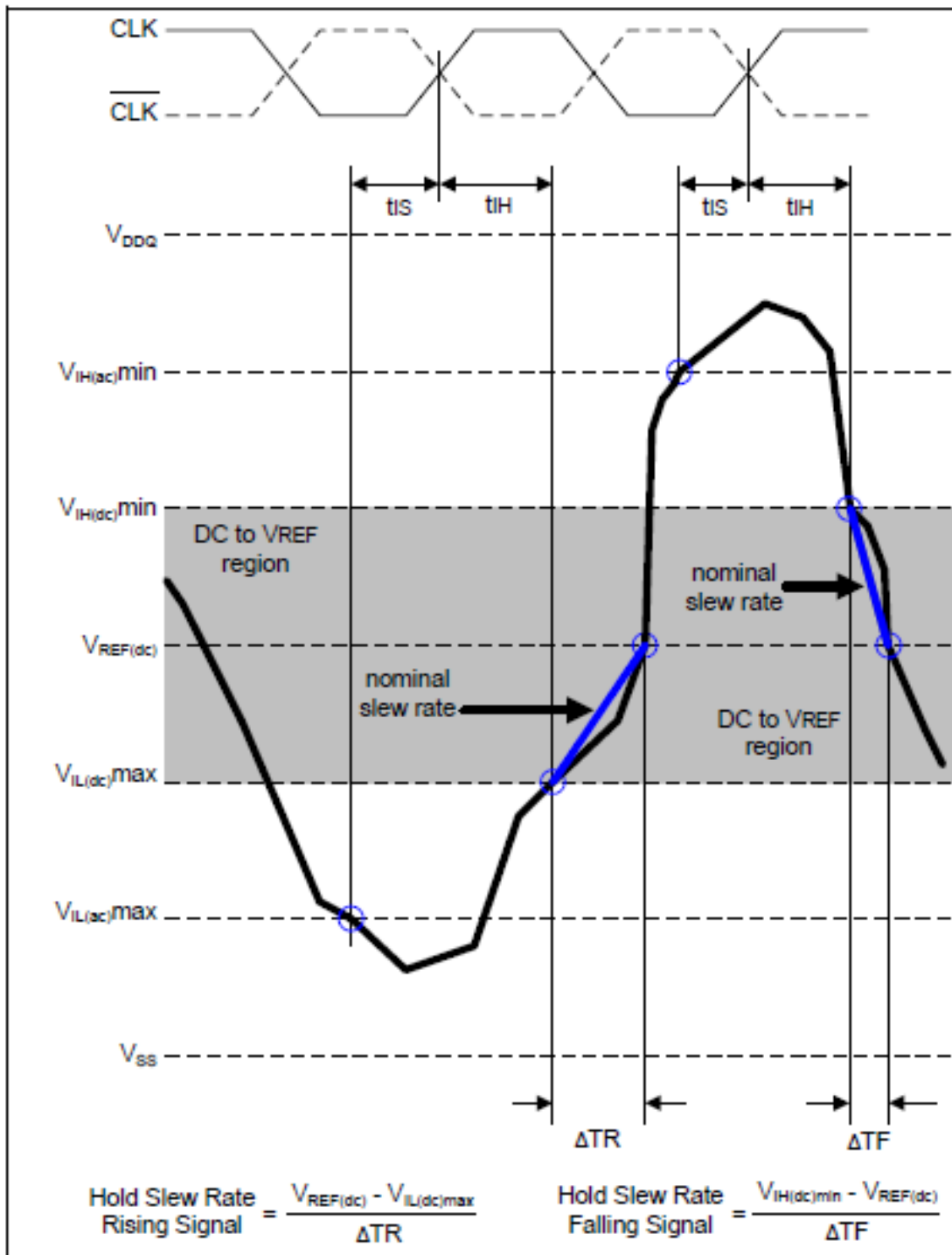
Figure 3 – Illustration of nominal slew rate for t IH
