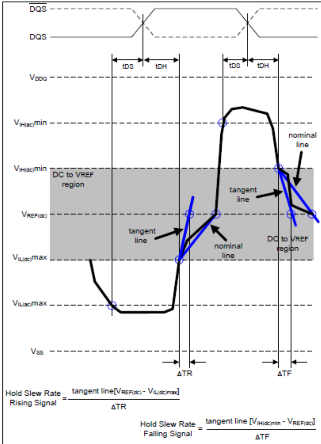
Figure 8 – Illustration tangent line for tDH (differential DQS, \overline{DQS} )
