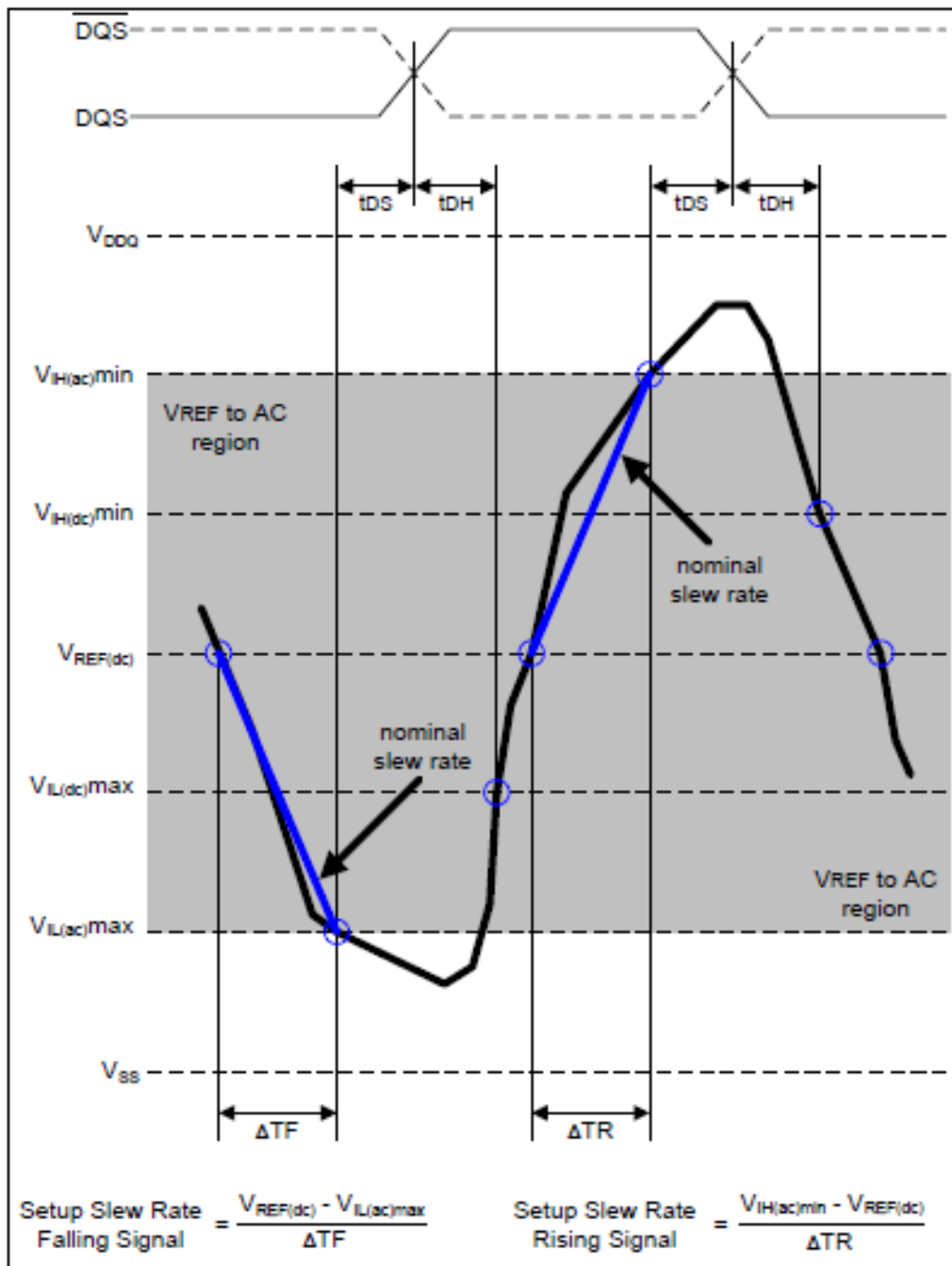
Figure 5 - Illustration of nominal slew rate for t_{DS} (differential \overline{DQS} , DQS )
