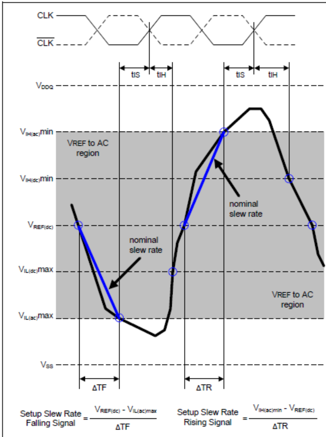
Figure 1 – Illustration of nominal slew rate for t_{IS}
