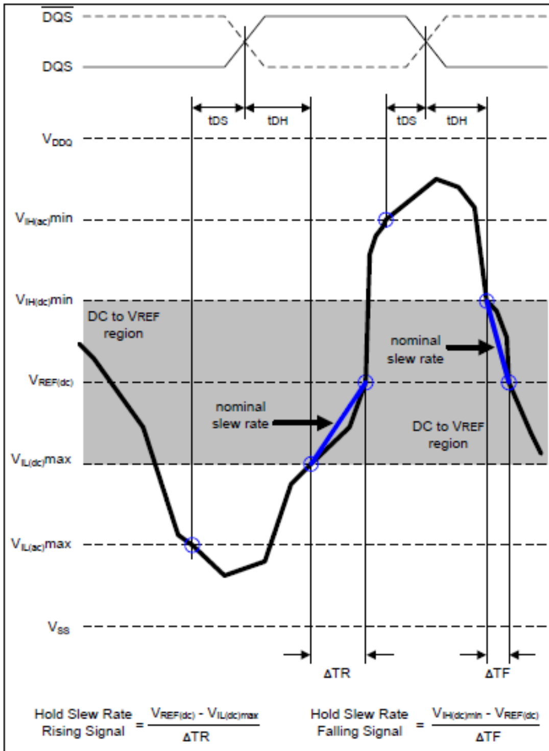
Figure 7 – Illustration of nominal slew rate for t DH (differential \overline{\text{DQS}} , \text{DQS} )
